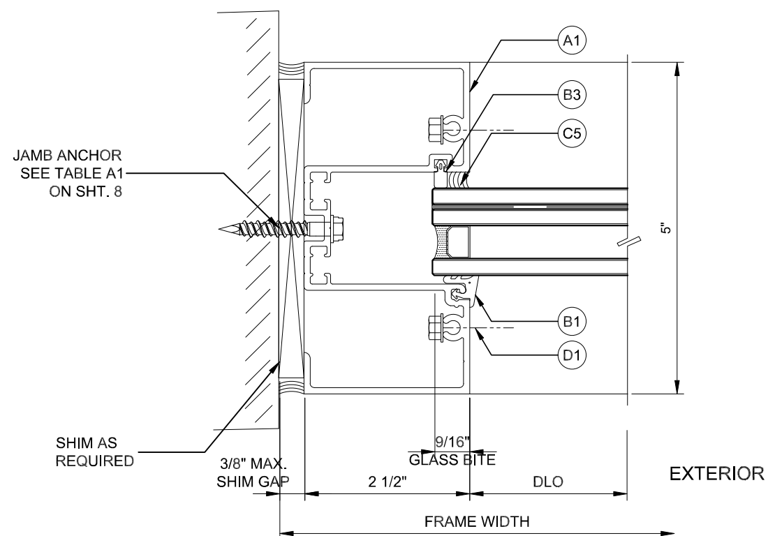
2 JAMB (ANCHORED)
