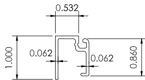
A13 3/8" GLASS STOP DF107
